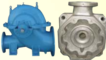
Pump Casings
